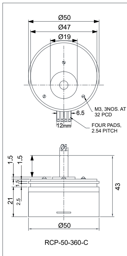
Dimensional Diagram
